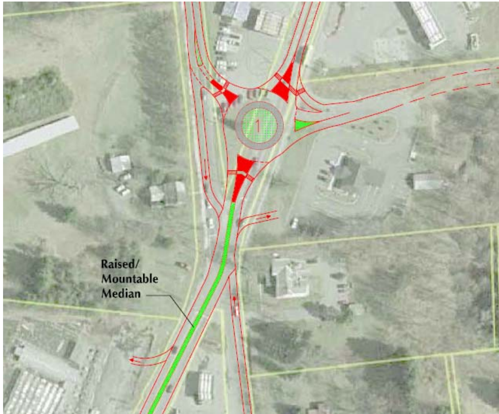
Roundabout concept for V-Corners at Routes 67 and 50 in the Town of Ballston, New York
