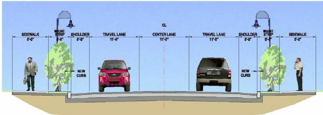
Potential Improvement for Broadway from Oakland Ave to Menands Road in the Village of Menands, New York.
